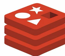
Databases
